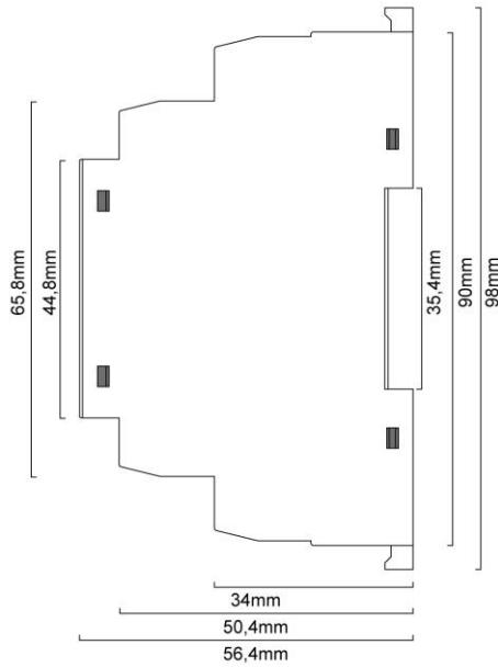
Geometrie RM16 HS
