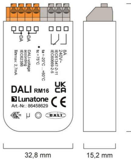
Geometrie RM8/RM16
